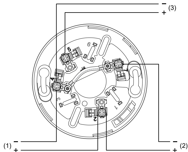
Figure 1: Wiring the KI-SB
